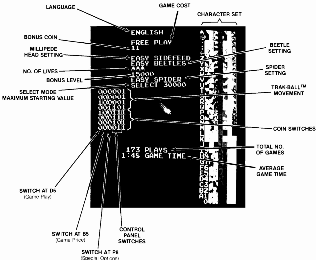
Figure 1-3 Self-Test Display
